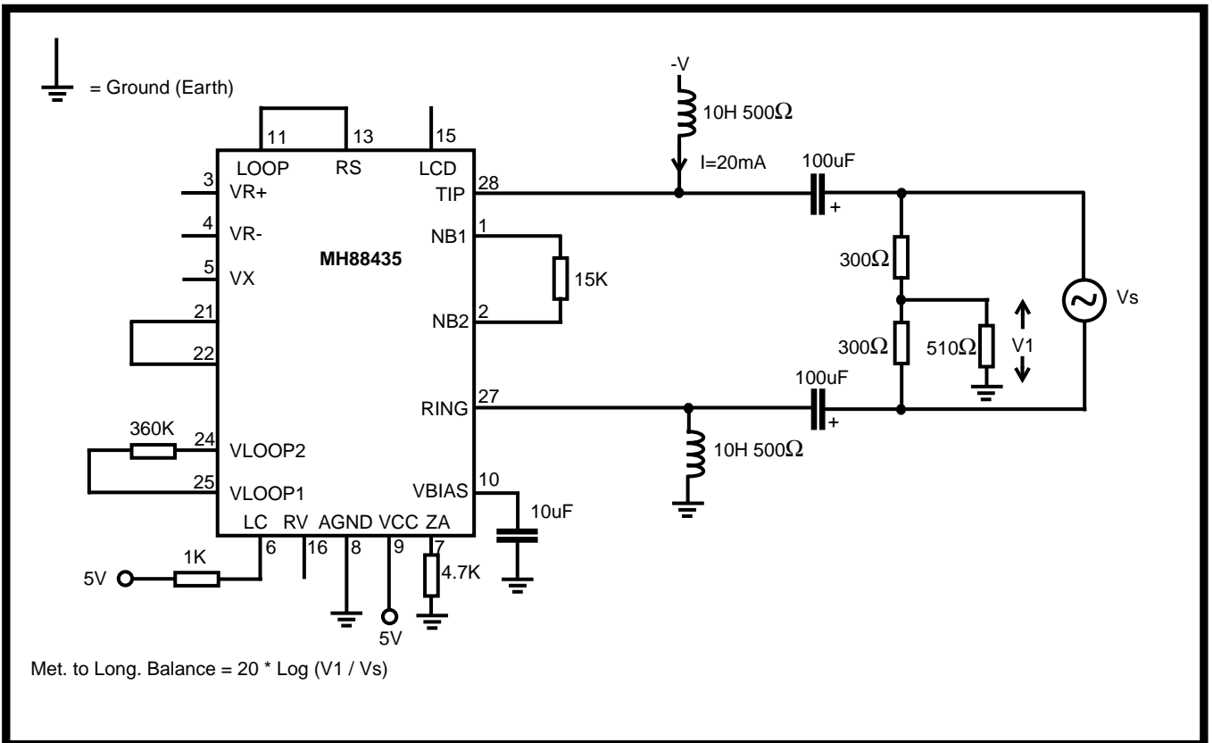
Figure 11 - Test Circuit 6
