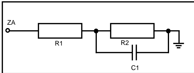
Figure 4 - Complex Impedances
