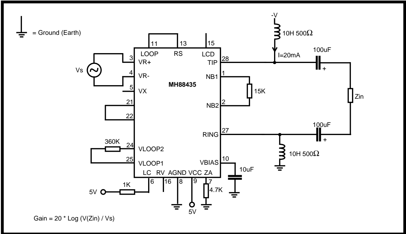
Figure 8 - Test Circuit 3
