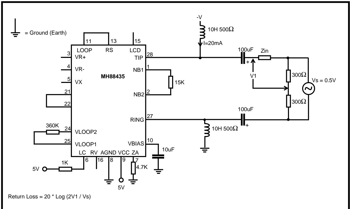
Figure 9 - Test Circuit 4
